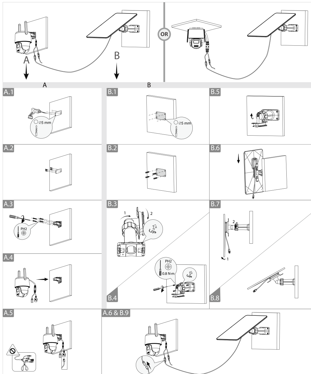
Figure 2-4 Attaching the camera and solar panel
