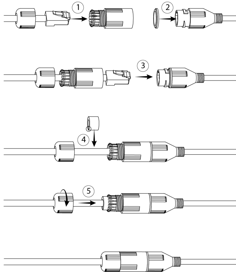
Figure 2-5 Install the waterproof connector
