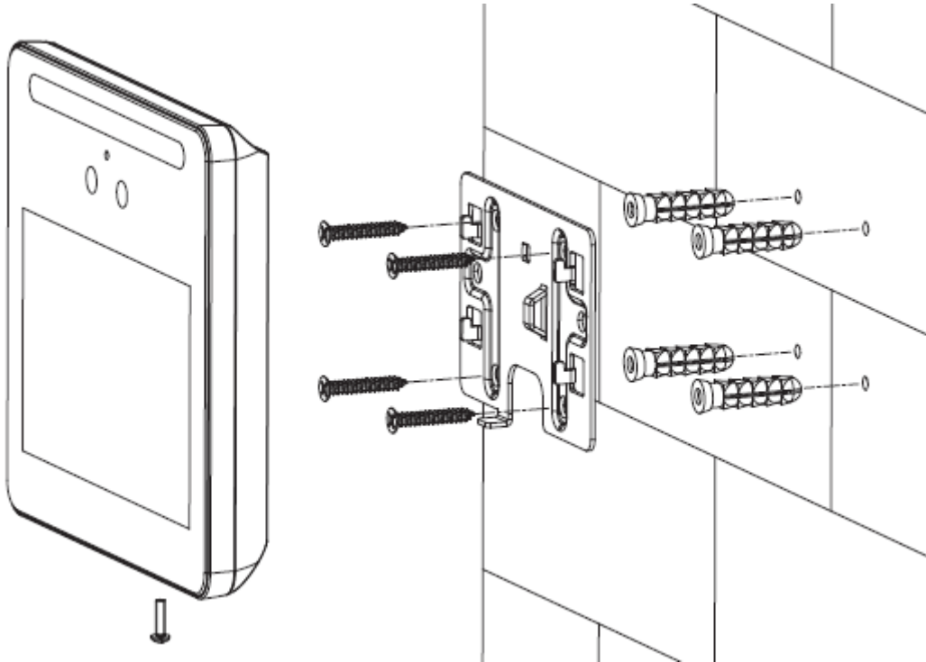
Figure 2-2 Wall installation
