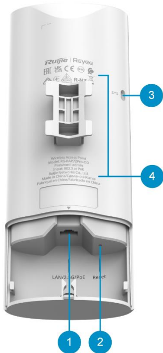
Figure 1-2 Rear Panel
